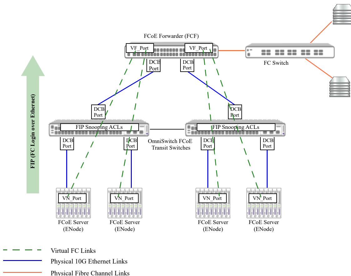
Figure 5-1 : OmniSwitch Transit Switch Connecting FCoE Endpoints
