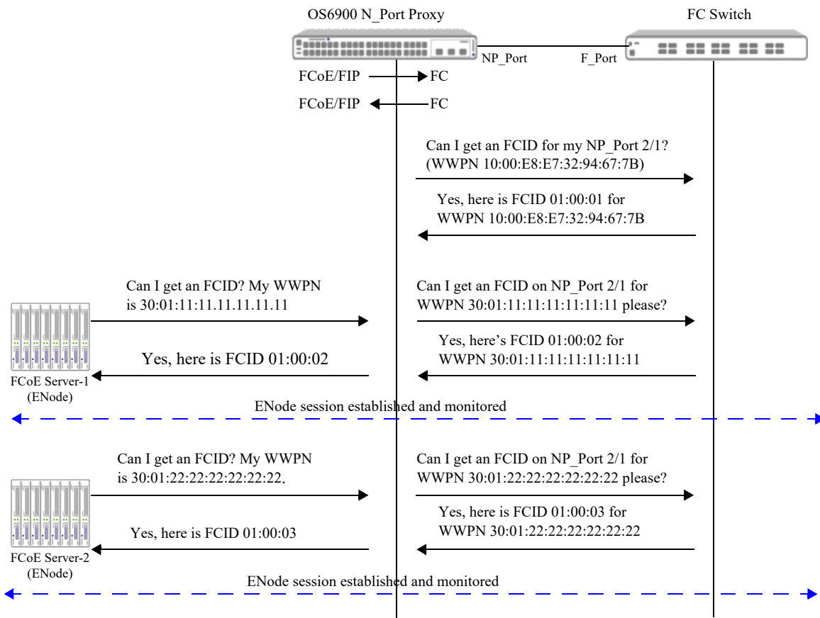
Figure 6-2 : OmniSwitch N_Port Proxy Overview
