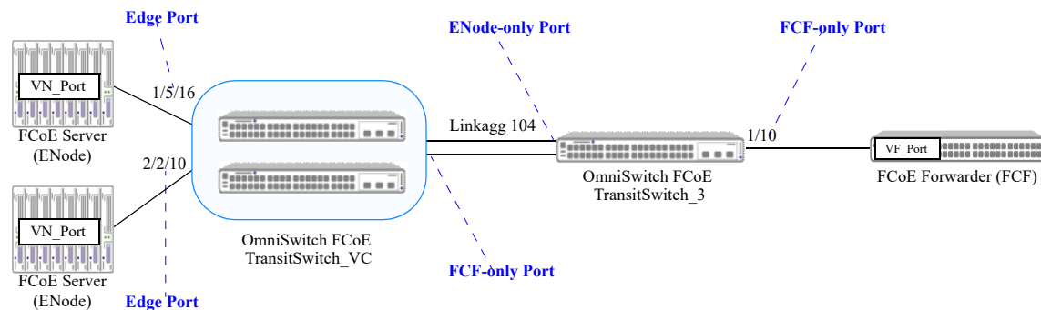
Figure 5-7 : Sample FCoE Topology
