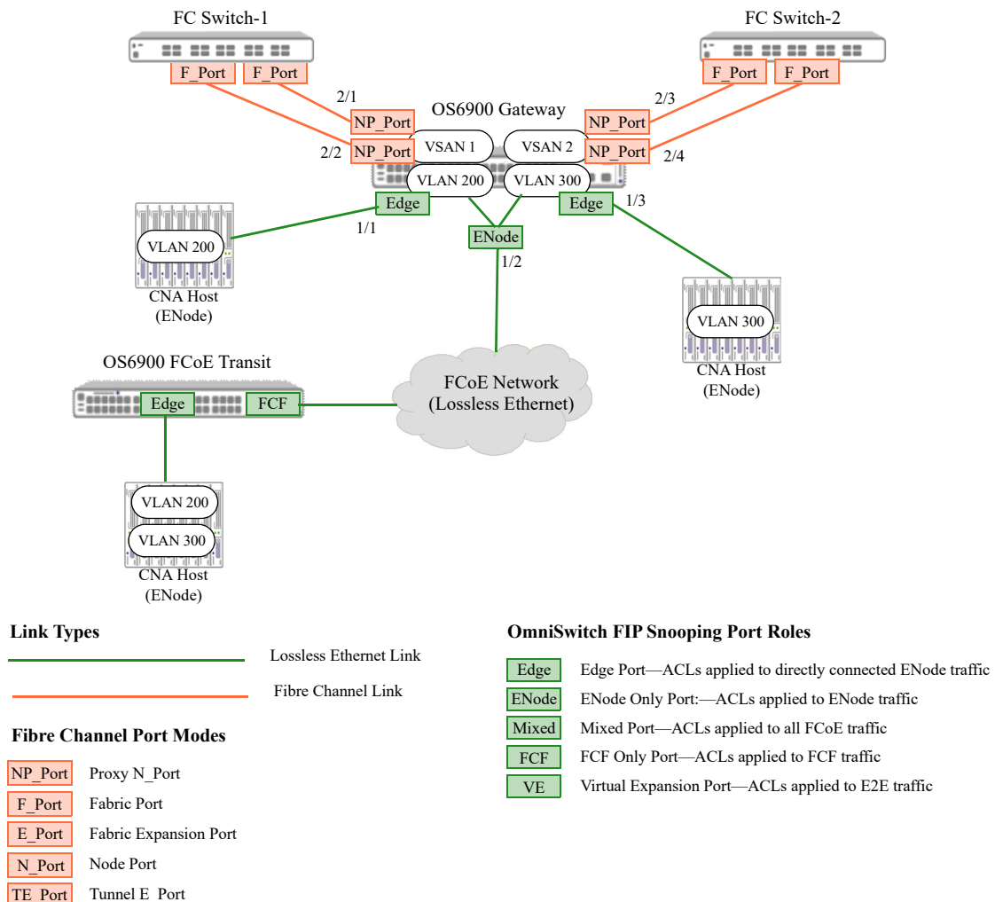
Figure 6-1 : OmniSwitch FCoE/FC Gateway Fabric
