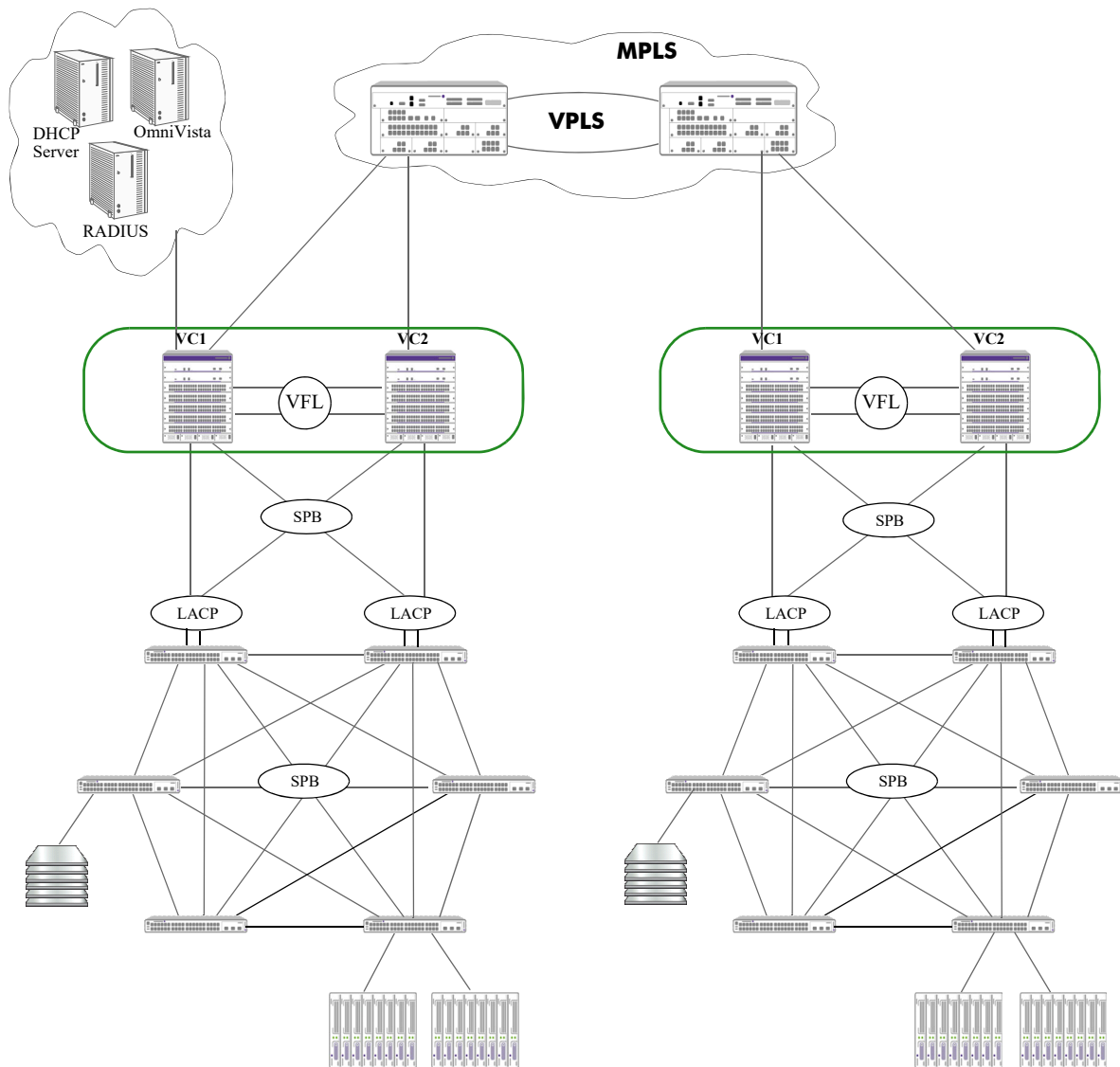
Figure 1-3 : Data Center Mesh Example
