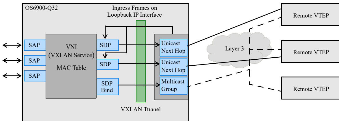
Figure 3-2 : OmniSwitch VXLAN Service Components
