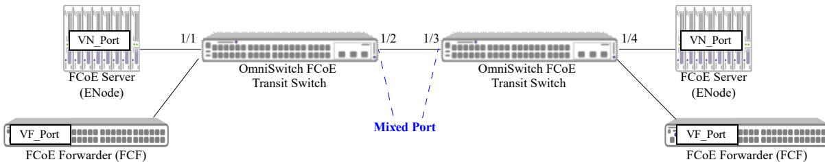
Figure 5-5 : FCoE Port Role-Mixed
