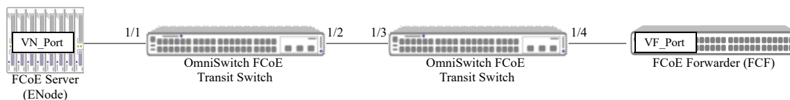
Figure 5-3 : FCoE Port Role-ENode
