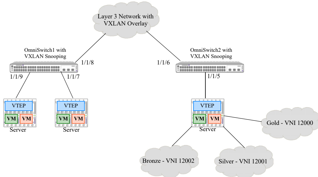
Figure 4-2 : VXLAN Snooping Configuration Example
