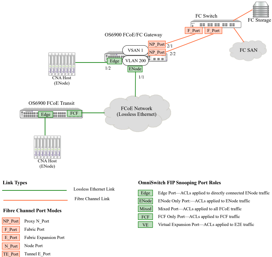
Figure 6-3 : OmniSwitch N_Port Proxy (NPIV) Example
